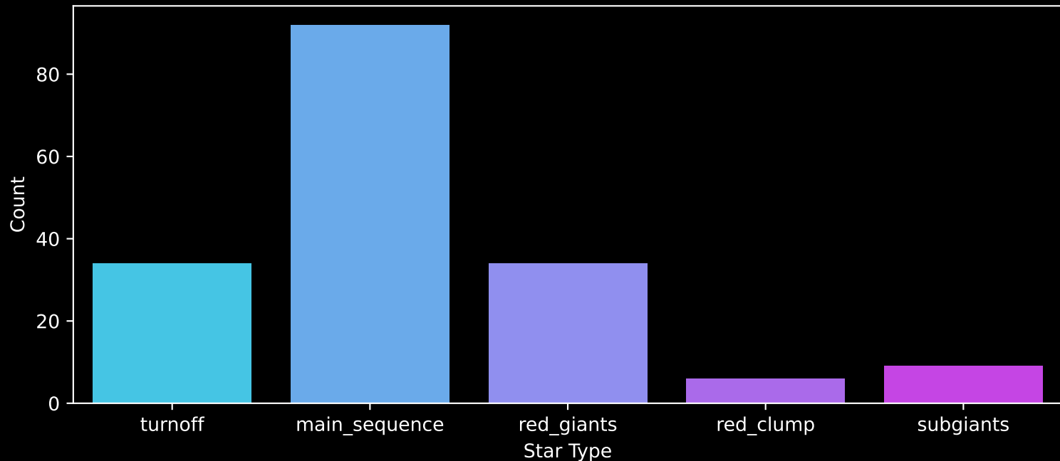
APOGEE DR17 Field: [044+42_MGA] Count plot of Star Type
